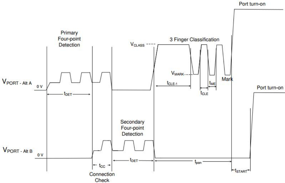
4-Pair single feature detection, 3 event classification and opening
