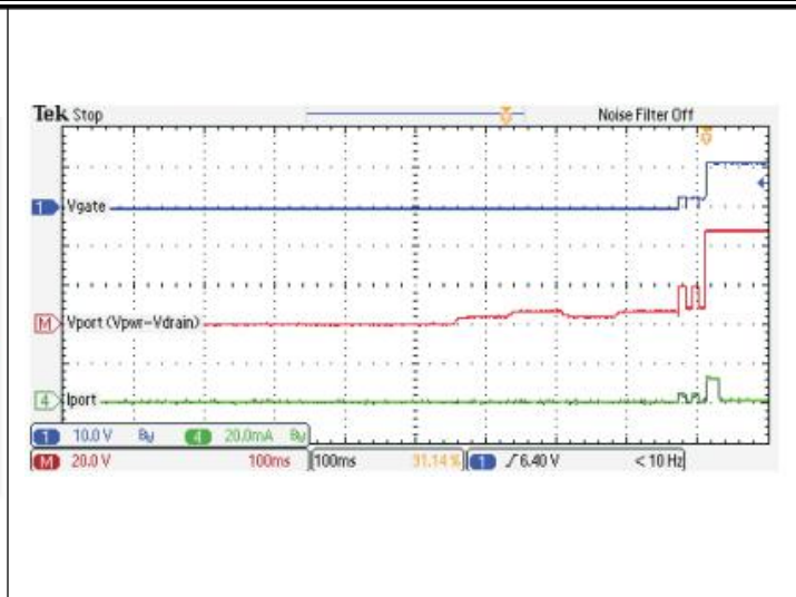
Event Class and Startup with Valid PD
