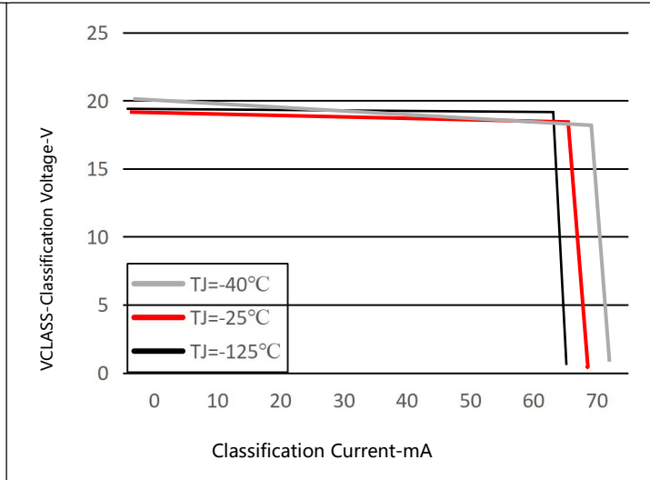
Classification Voltage vs Port Classification Current
