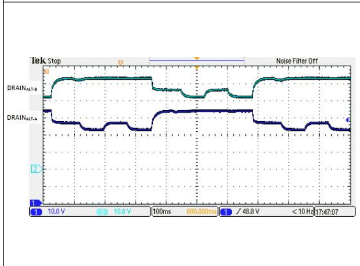
Detection characteristics of 4-Pair high resistance (36K Ω)
