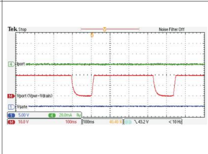
Detection characteristics of 4-Pair low resistance (11K Ω)
