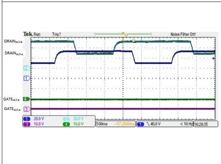
4 - line pair open - circuit detection features
