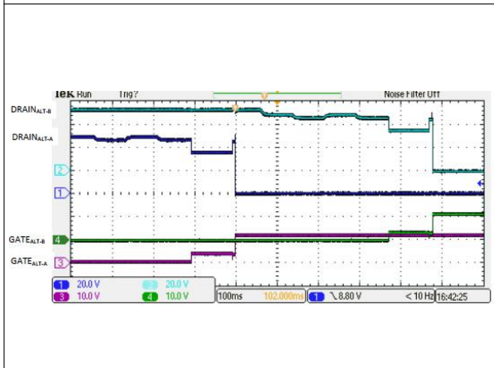
4-Pair dual feature 1 finger grading and opening
