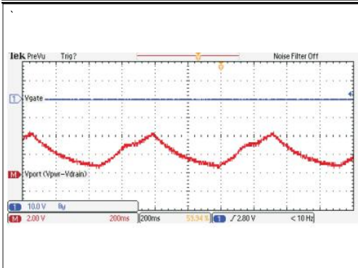
Detection with Invalid PD (25 kΩ and 10 μF)
