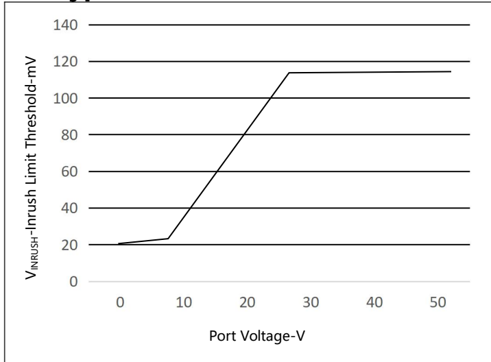
Inrush Current Limit Threshold vs Port Voltage
