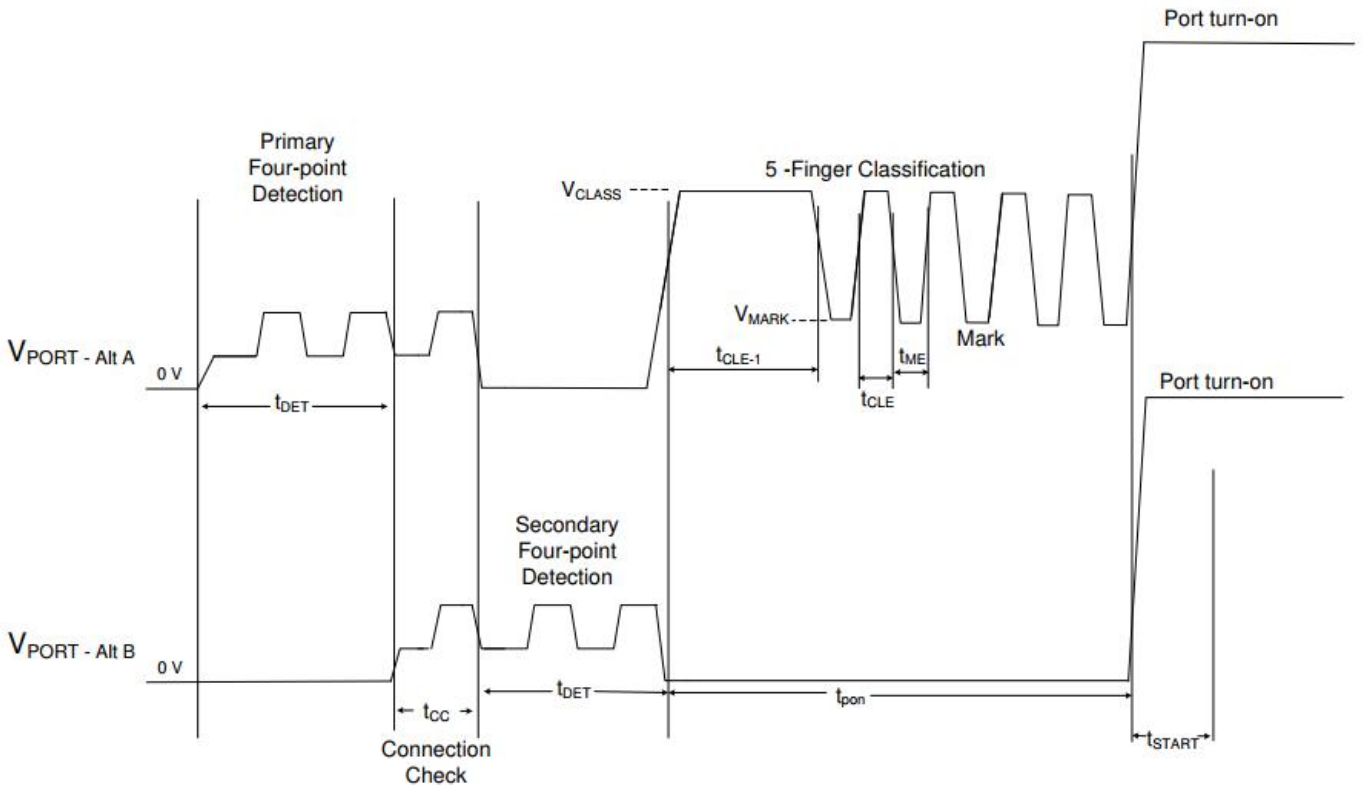
4-Pair single feature detection, 5 event grading and opening
